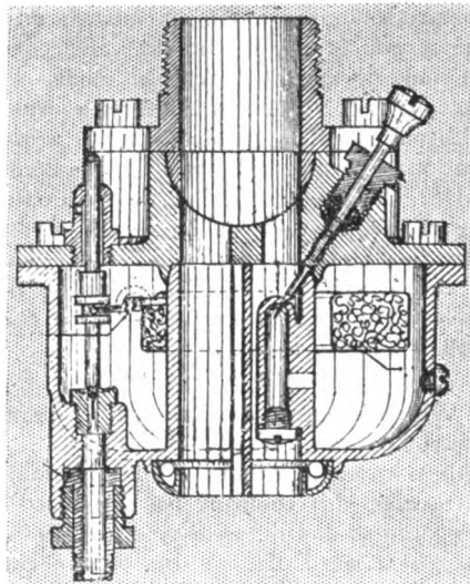
Allen Two-Port Carbureter.
